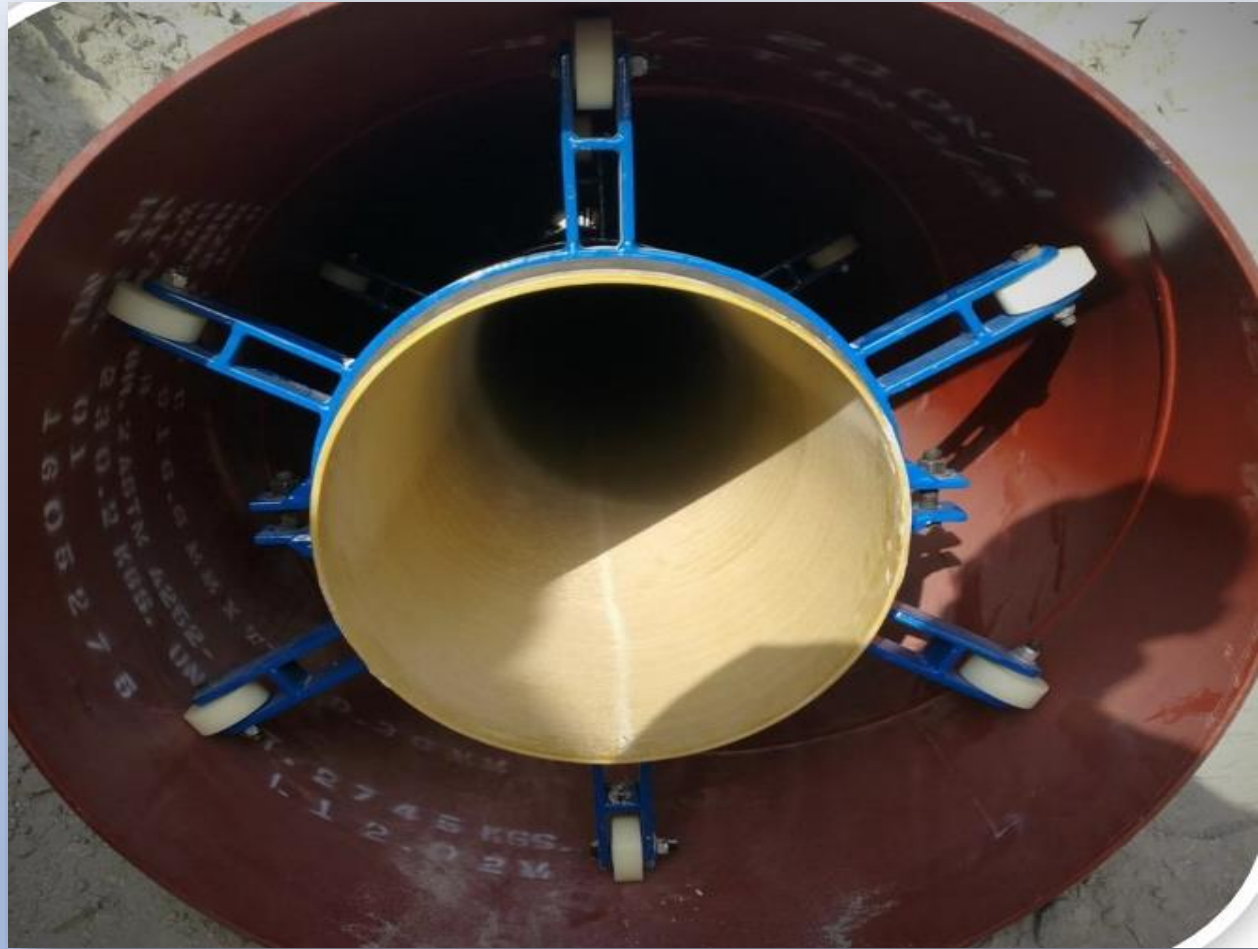
Non-Destructive Road Crossing (NDRC) for DEWA Water
